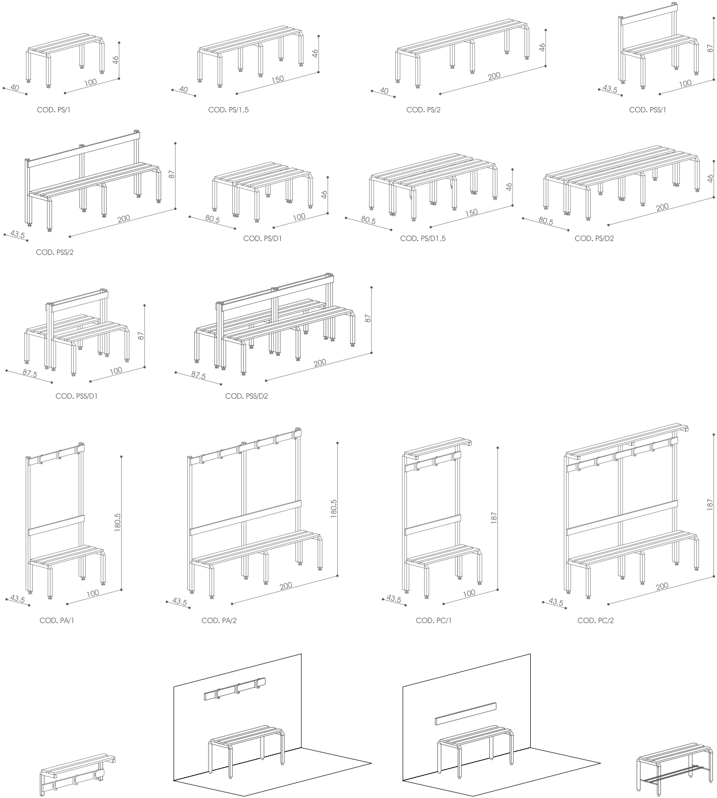
Attaccapanni da muro, con portaborse Wall coat hanger with bag-rack
